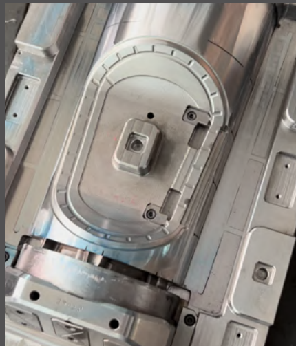
POTTIES IN PRODUCTION 800KG HEAVY DIAPER BIN STEEL MOULD
